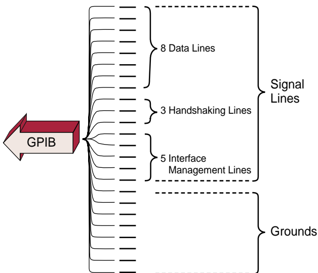
Figure 2. GPIB Signals and Lines
