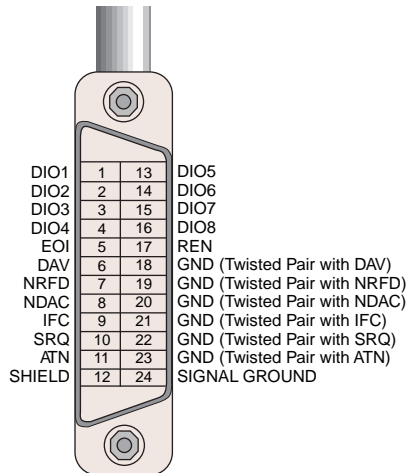
Figure 3. GPIB Connector and Signal Assignment
