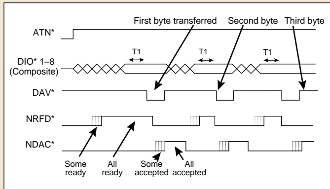
Figure 7. Normal IEEE 488.1 Handshake
