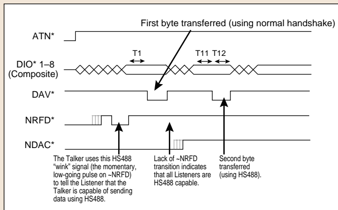
Figure 8. HS488 Handshake
