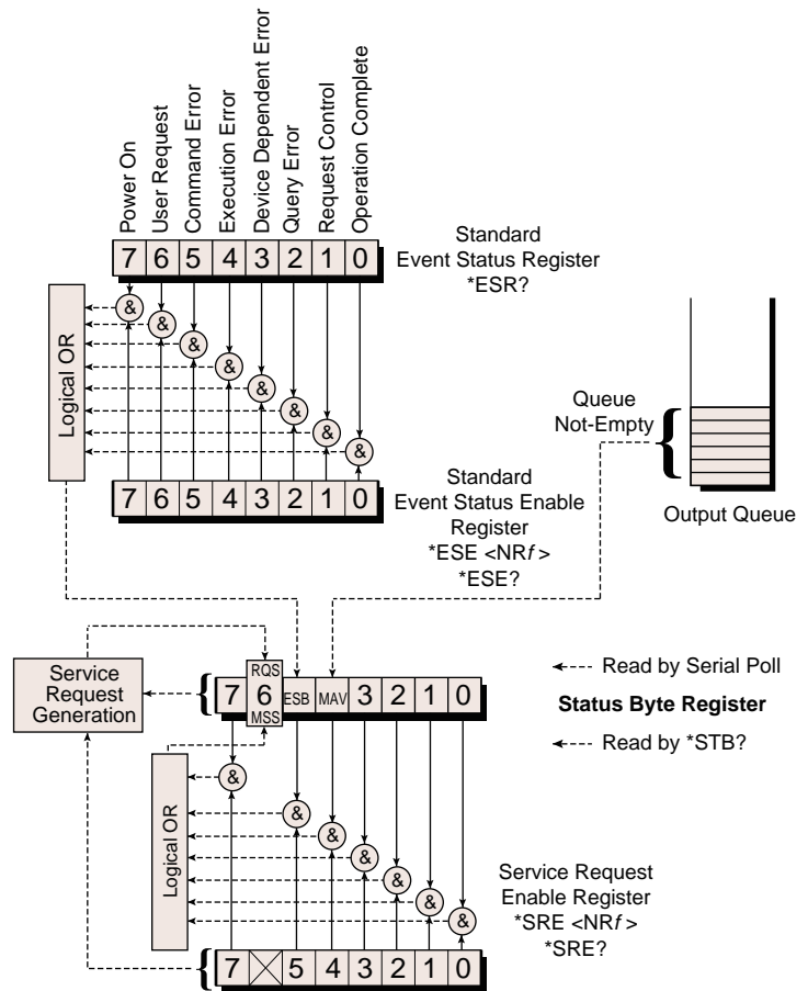
Figure 9. Status Report Model
