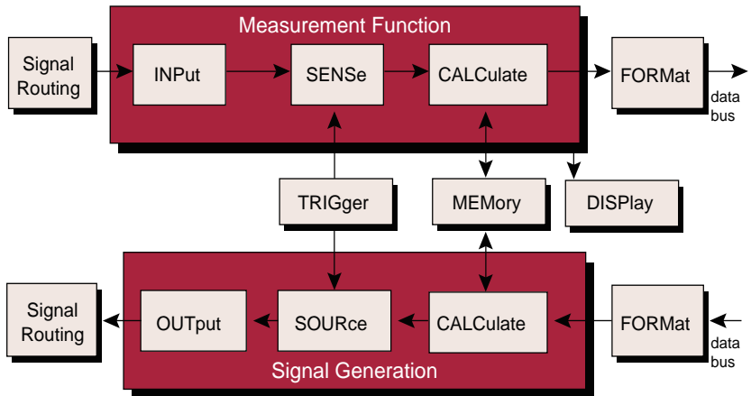
Figure 10. The SCPI Instrument Model
